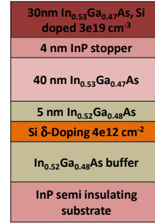
Fig. 1. Starting heterostructure
