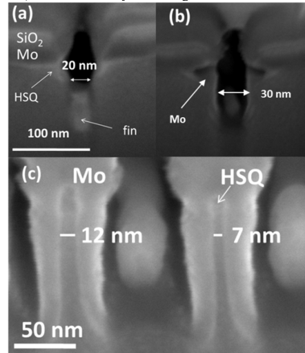
Fig. 6. FIB cross-section of finished device from source to drain: (a) along fin and (b) between the fins; (c) Cross-section FIB of two completed fin test structures.
